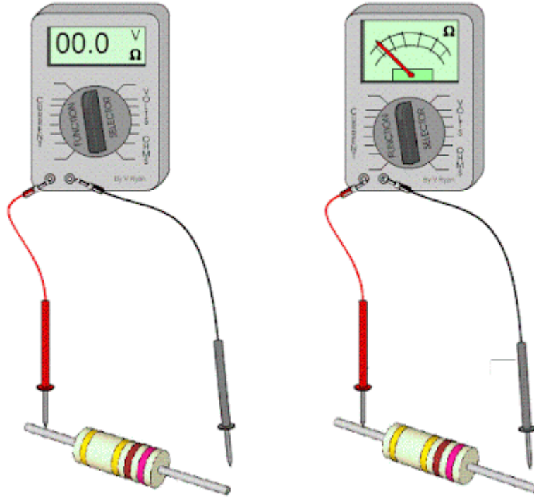
Ohmmetre
